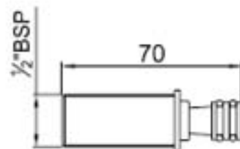
SPOUT NIPPLE
