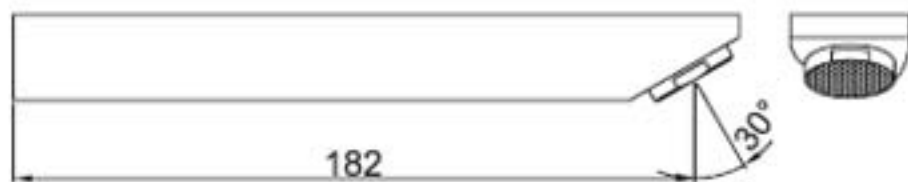
SPOUT
