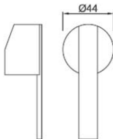
HANDLE
