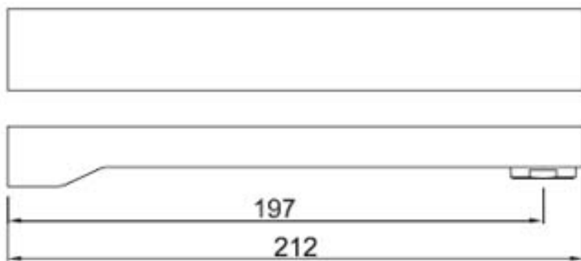
SPOUT
