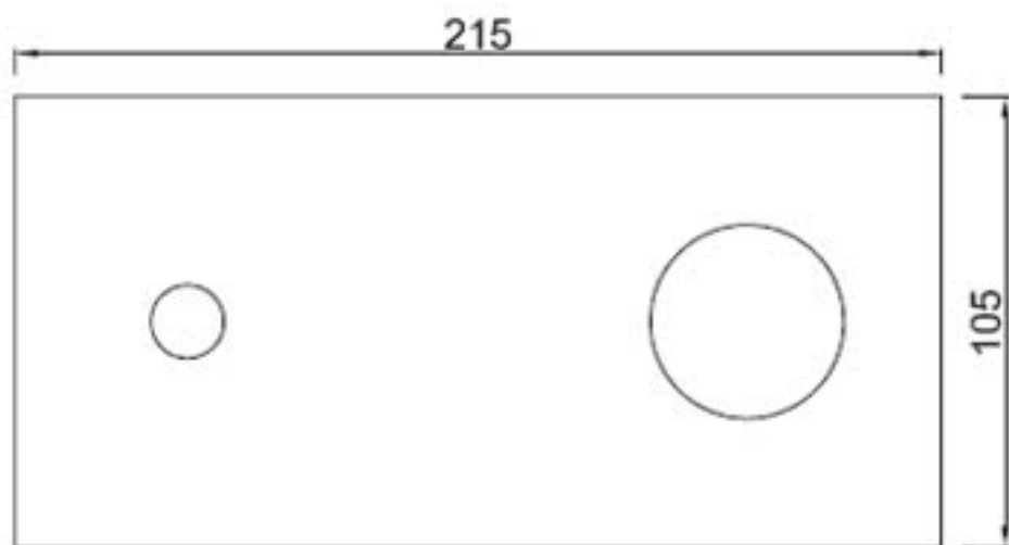
WALL FLANGE
