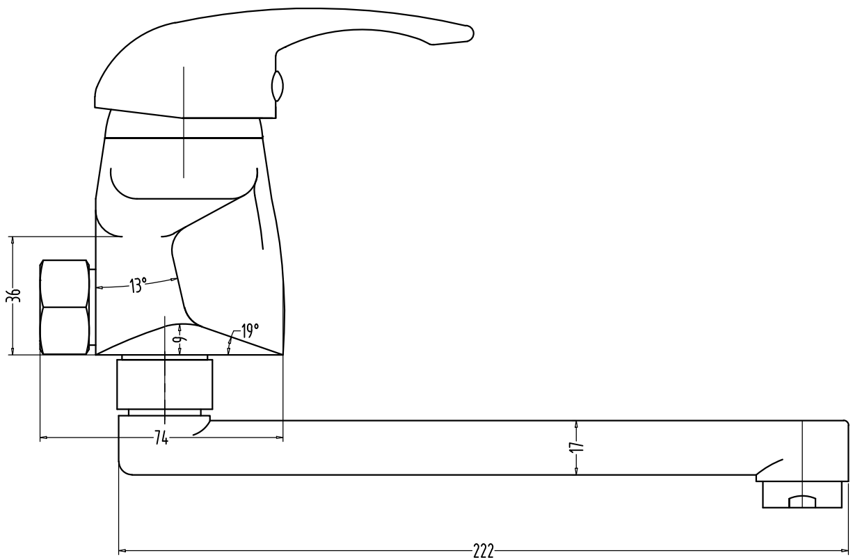
ESSENCE F130013 S/L SINK MIXER WITH SWIVEL SPOUT (WALL MOUNTED MODEL)
