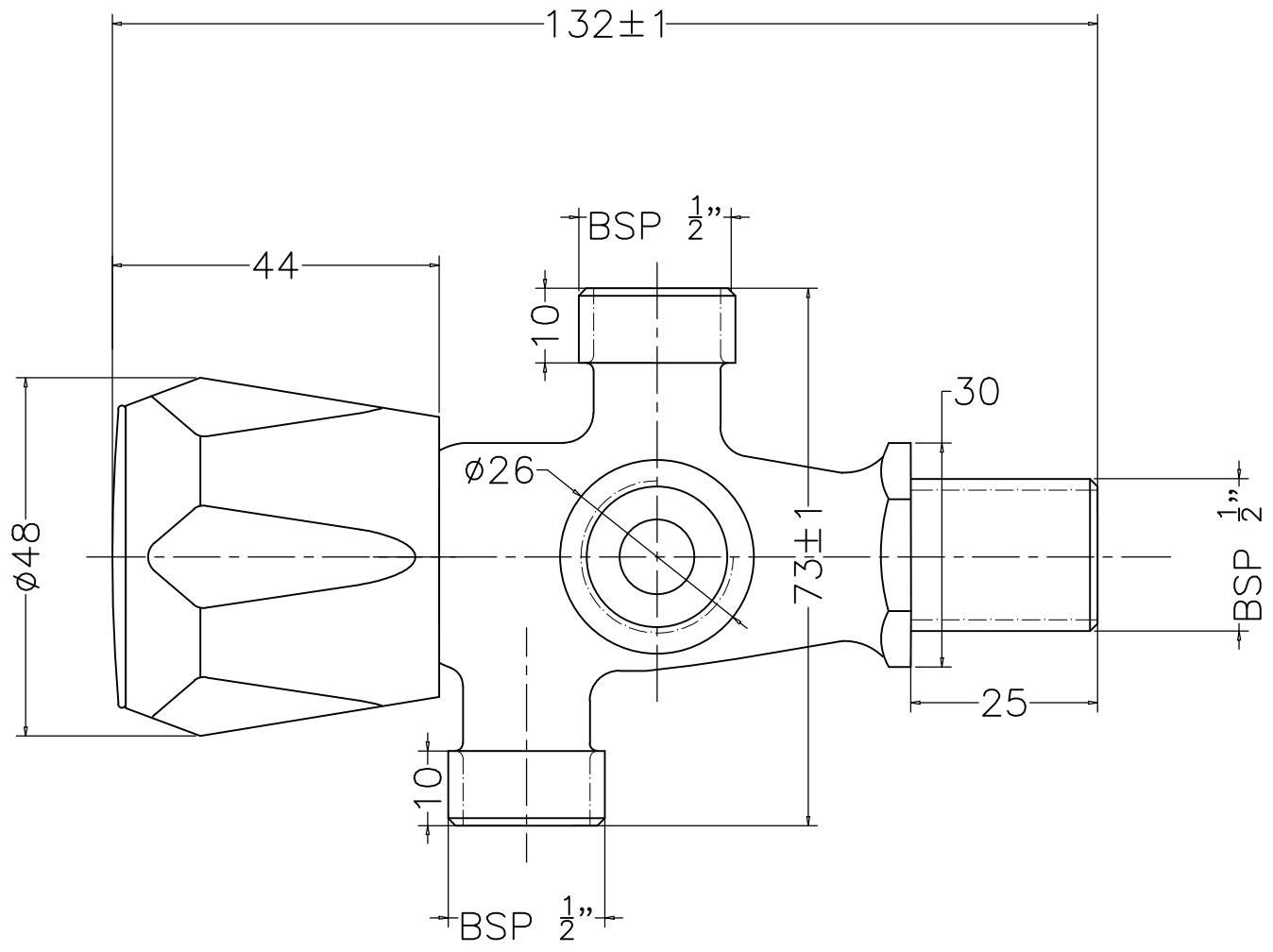
CLASSIK F200006 ANGULAR STOP COCK - 2 Way
