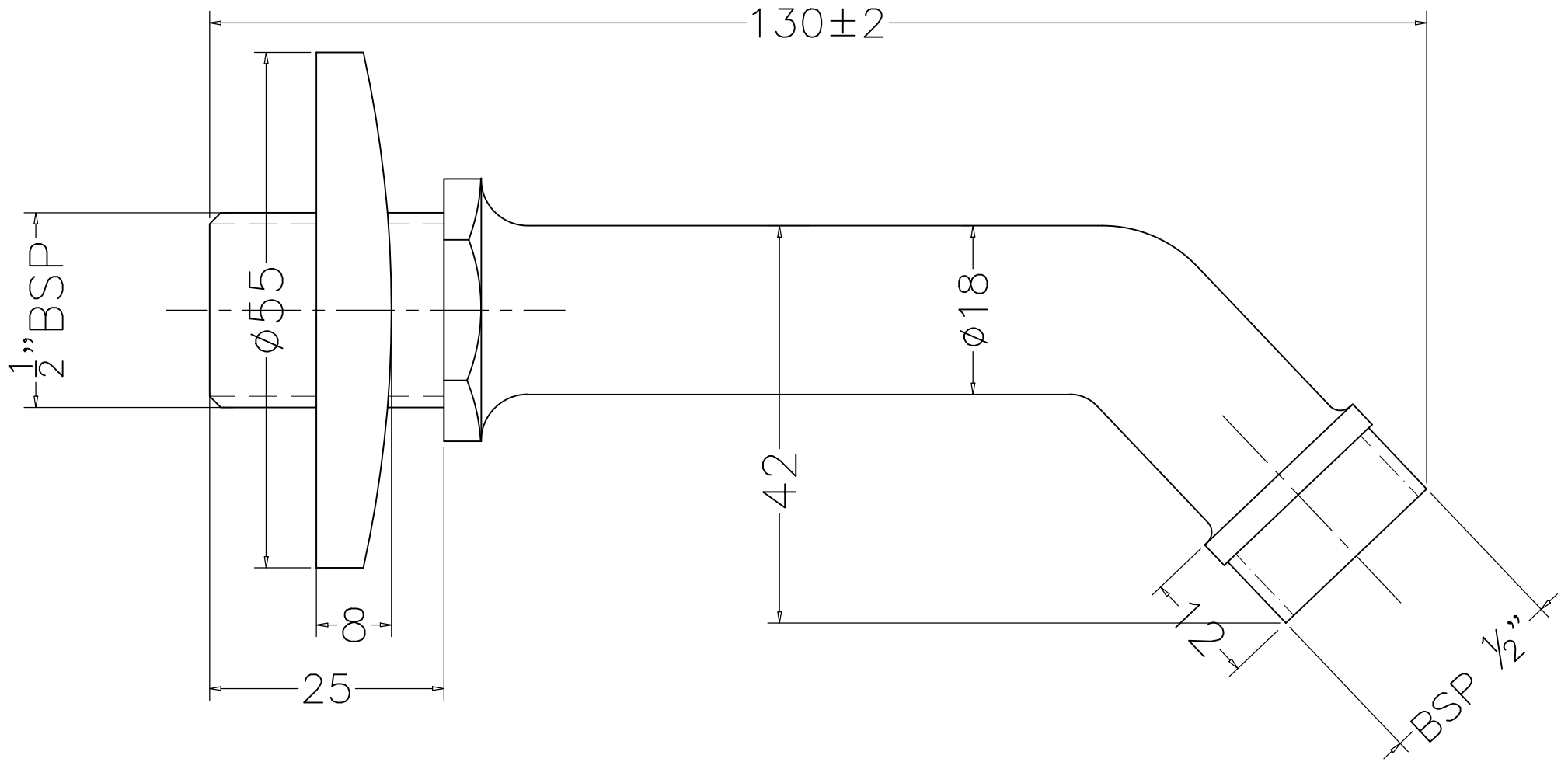
CLASSIK F200028 SHOWER ARM LIGHT WITH FLANGE
