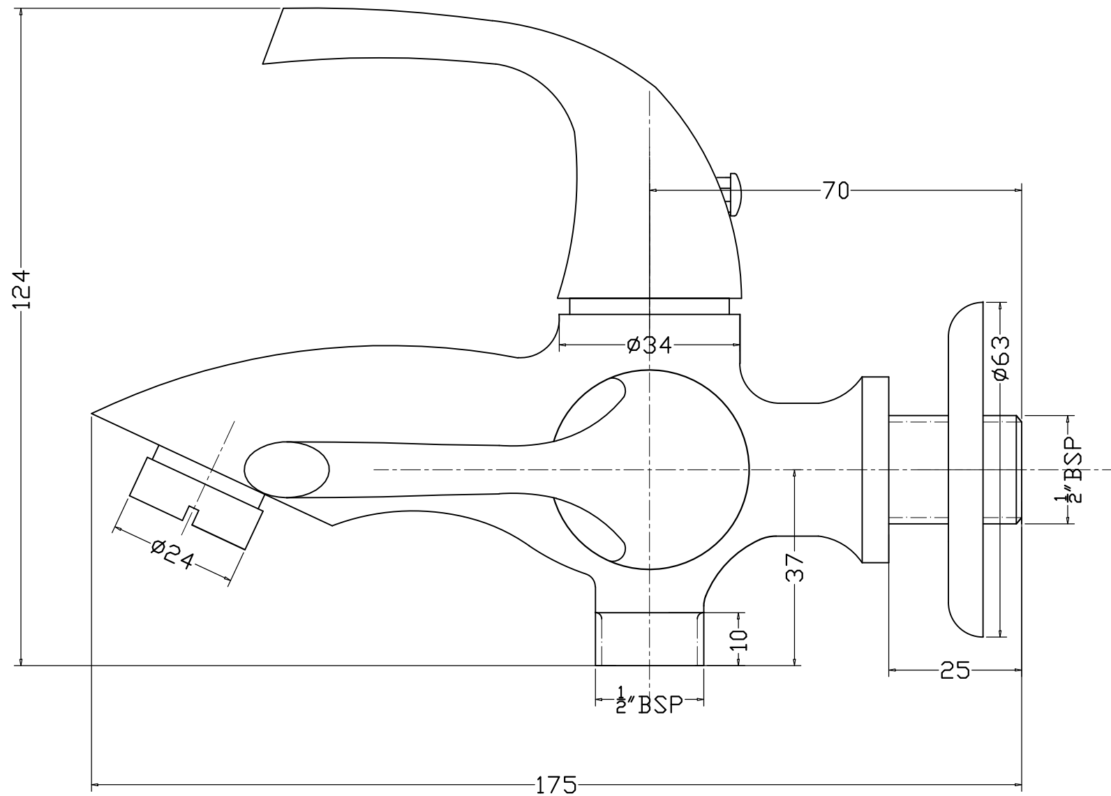
GRACCIA F250003 BIB COCK 2 IN 1 WITH WALL FLANGE
