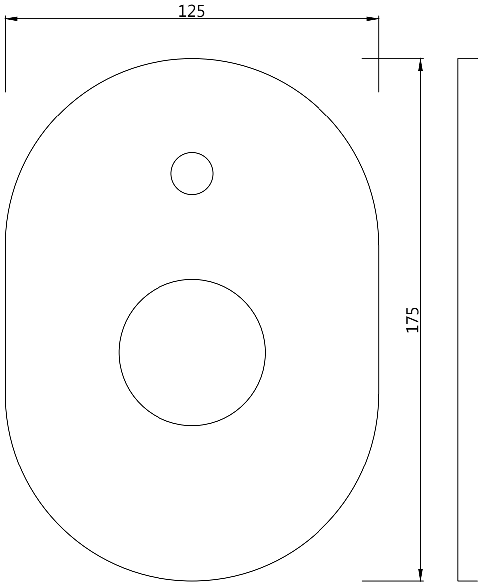
WALL FLANGE
