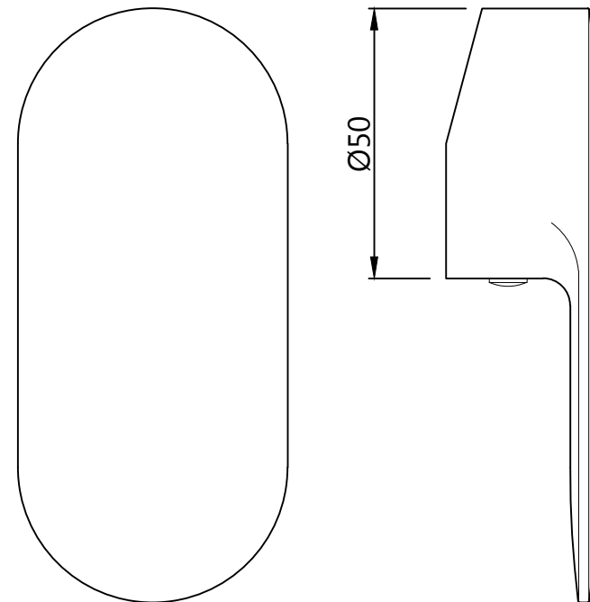
HANDLE
