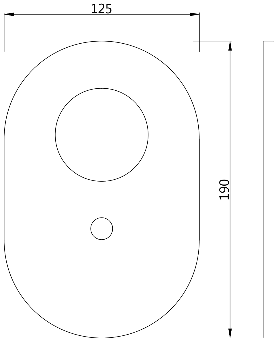
WALL FLANGE
