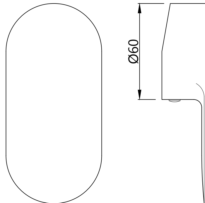
HANDLE
