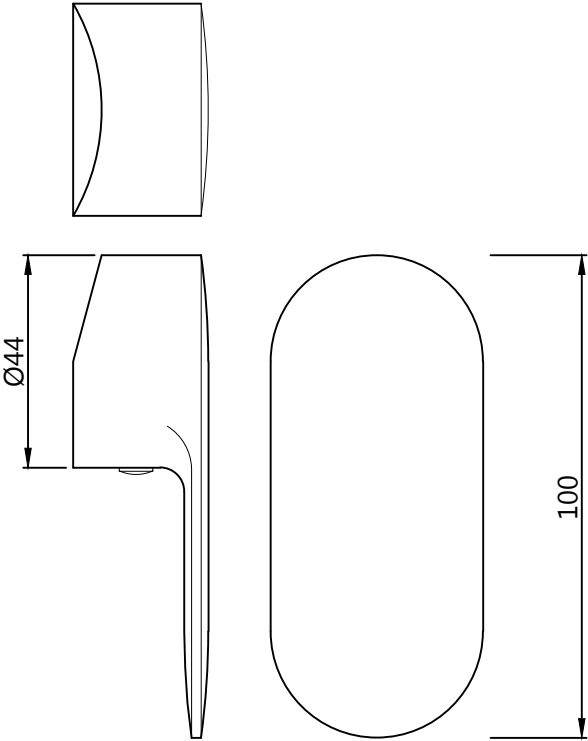
HANDLE
