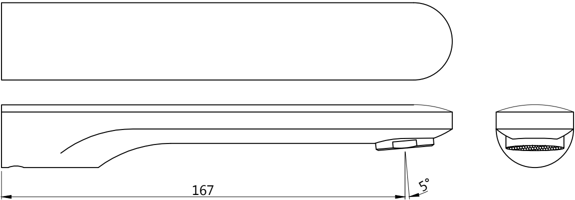
SPOUT
