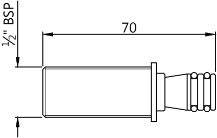
SPOUT NIPPLE
