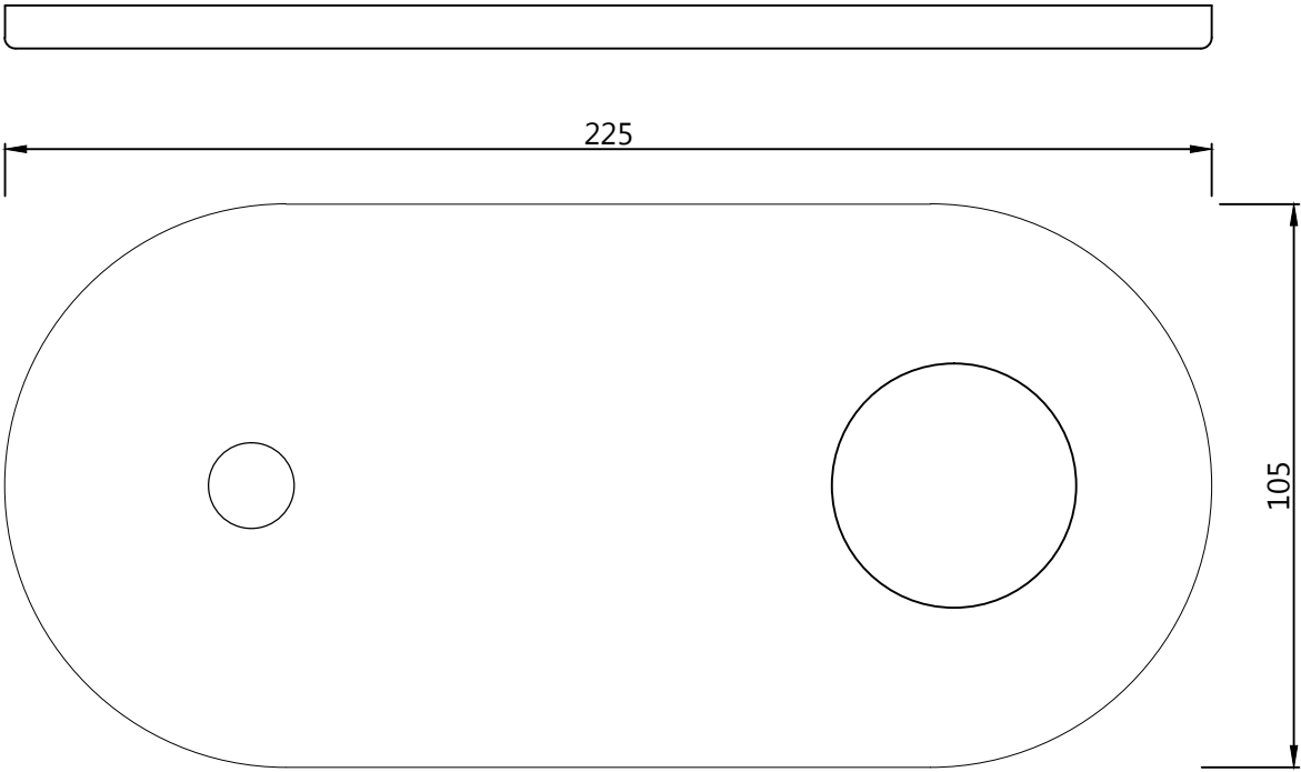
WALL FLANGE
